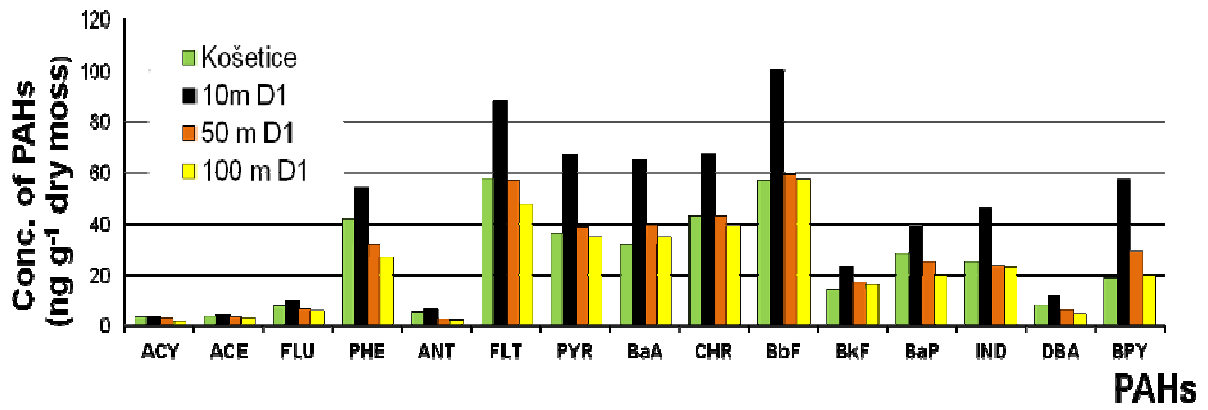
Fig. 6 Concentration of selected PAHs in moss in distance up to 100 m from the highway D1 (km 36) and at the reference plot Košetice.
