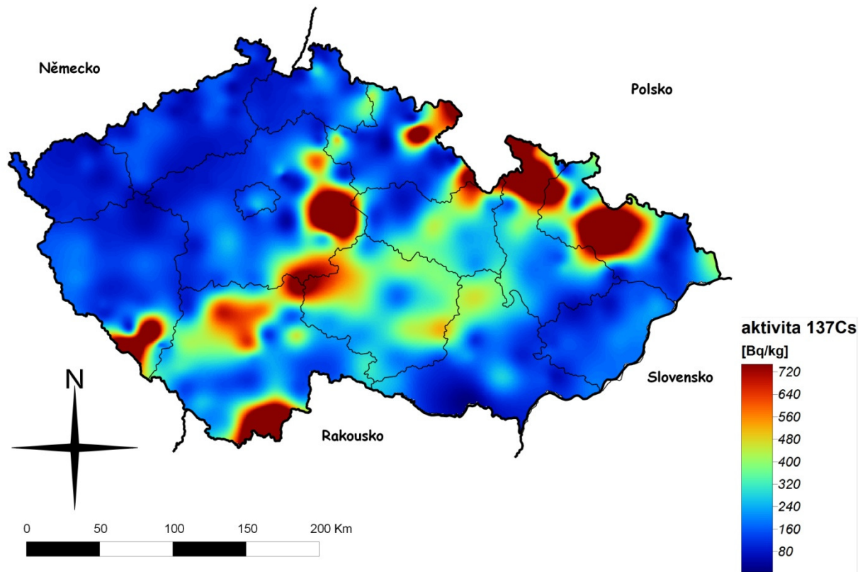
Fig. 9 Content of ^{137}\text{Cs} in forest floor humus in the Czech Republic in 2005.
