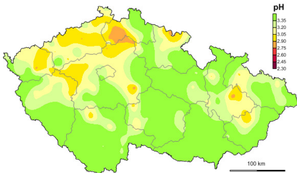
Obr. 5 Reaction (pH) of spruce bark extract in the Czech Republic in 2010.
